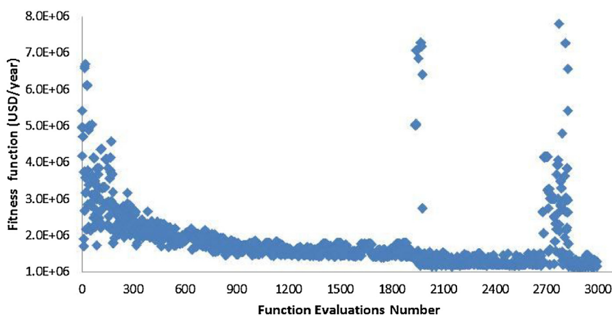
Fig. 6 – Generalized trend of the optimization process.
