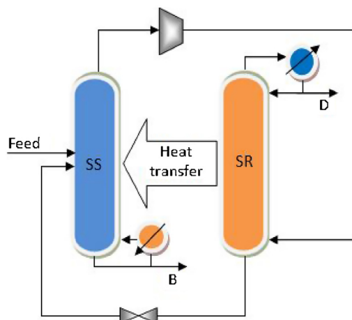
Fig. 2 – HIDiC configuration.
